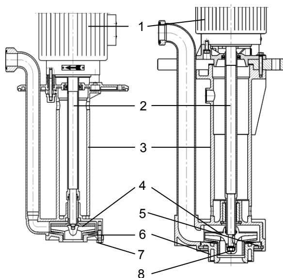
Fig. 9 Cross-section of F 716 PP1-... (sample view)
