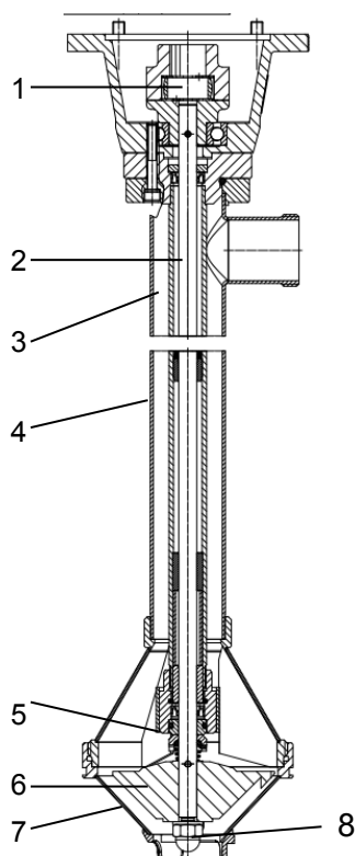
Fig. 1 Cross-section of F 620 S-15, F 620 S-30 (sample view)
