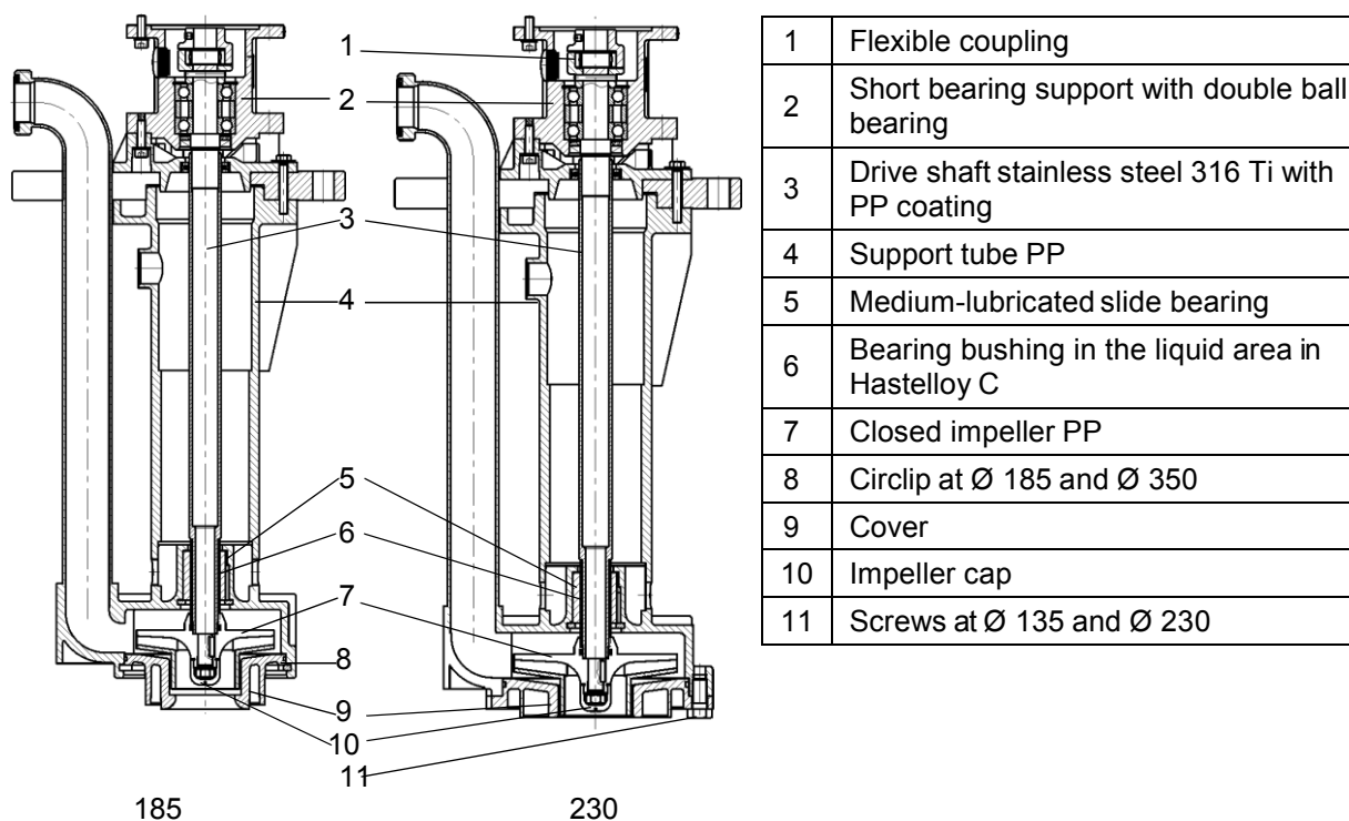
Fig. 8 Cross-section of F 706 PP-... (sample view)
